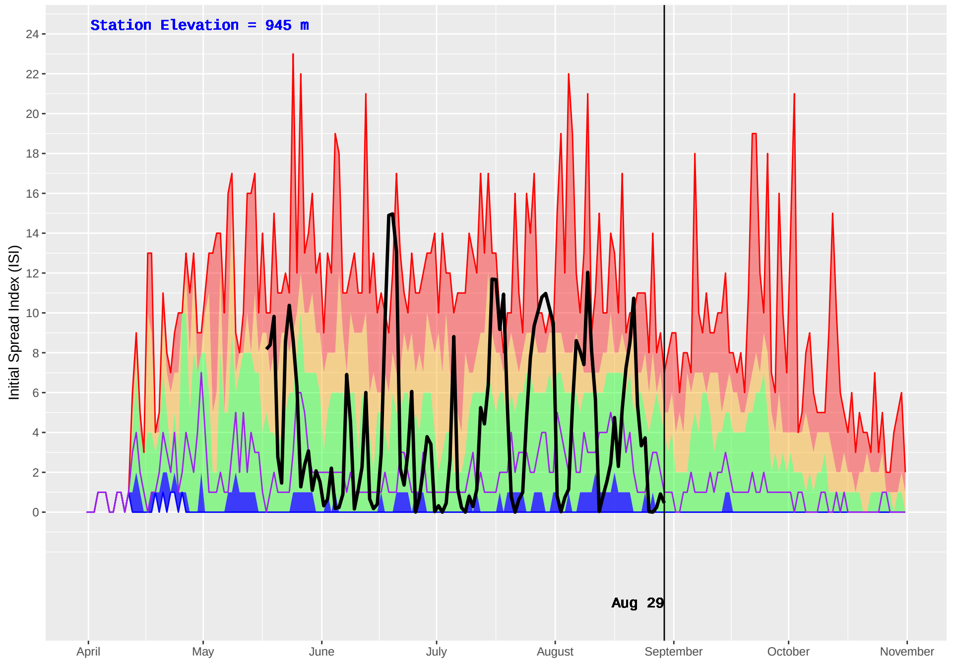
BOWRON HAGGEN (193) : Historical (1986–2016) and Current (2018) Daily Initial Spread Index (ISI)
