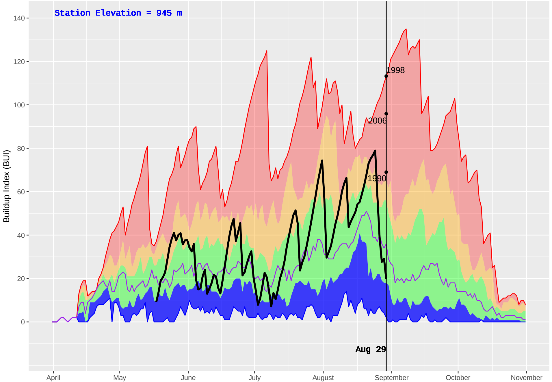
BOWRON HAGGEN (193) : Historical (1986–2016) and Current (2018) Daily Buildup Index (BUI)
