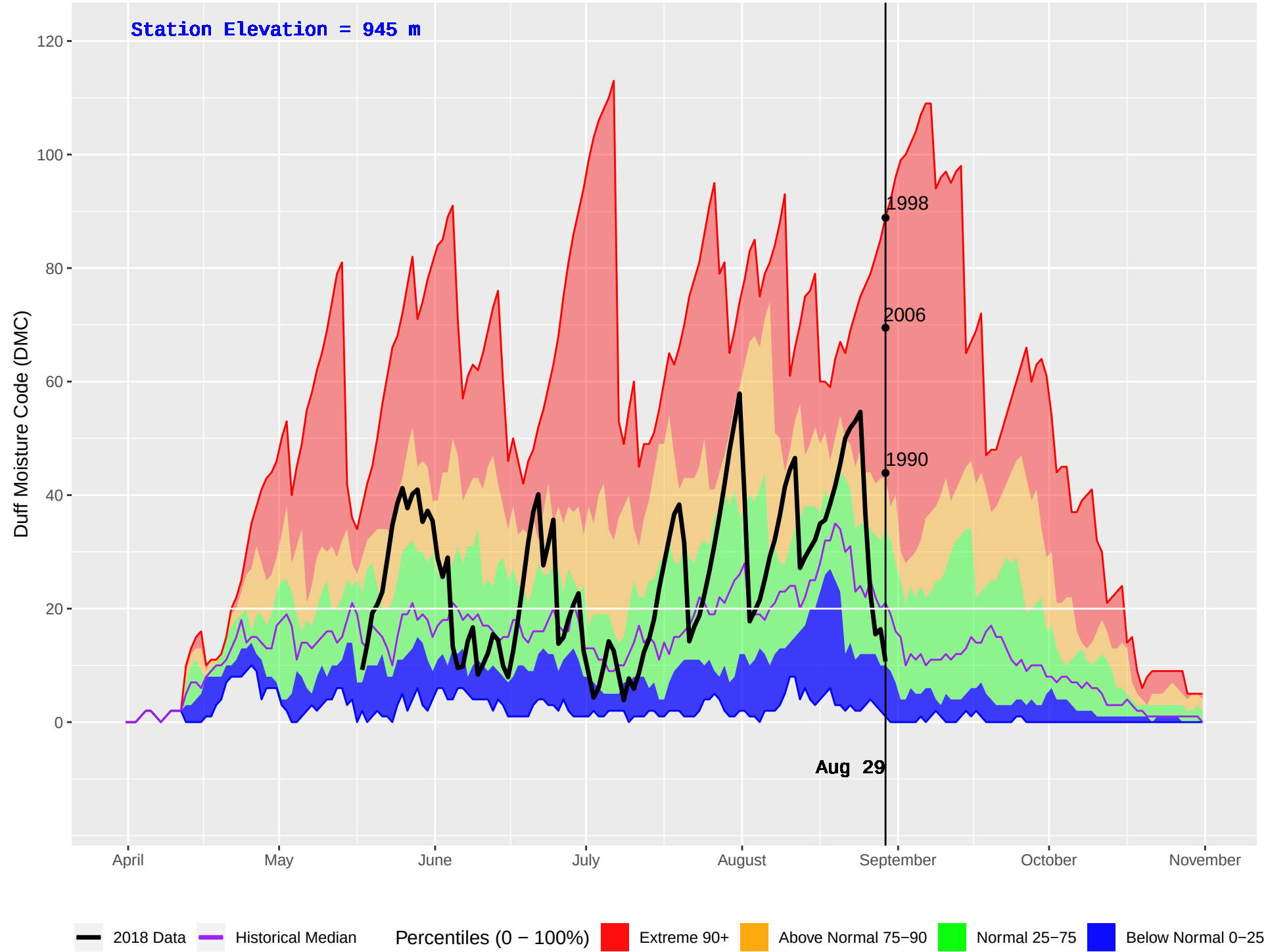
BOWRON HAGGEN (193) : Historical (1986–2016) and Current (2018) Daily Duff Moisture Code (DMC)
