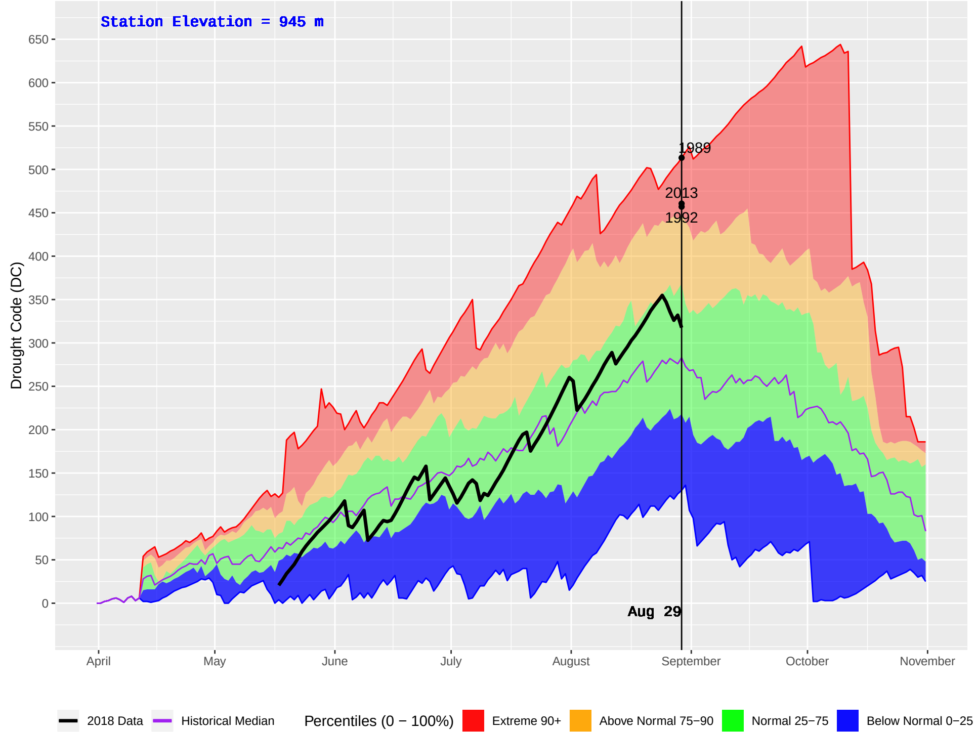
BOWRON HAGGEN (193) : Historical (1986–2016) and Current (2018) Daily Drought Code (DC)
