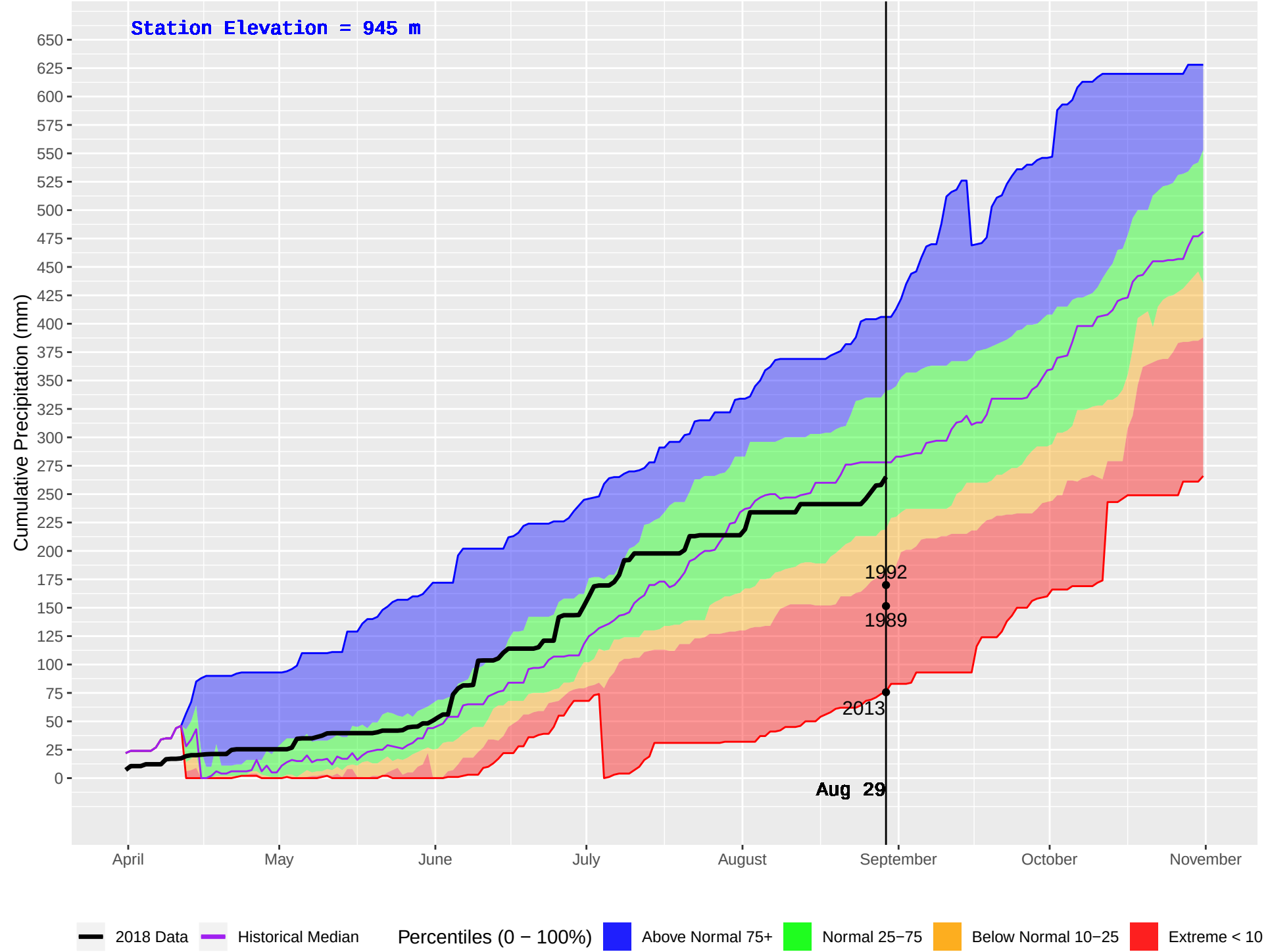
BOWRON HAGGEN (193) : Historical (1986–2016) and Current (2018) Daily Cumulative Precipitation
