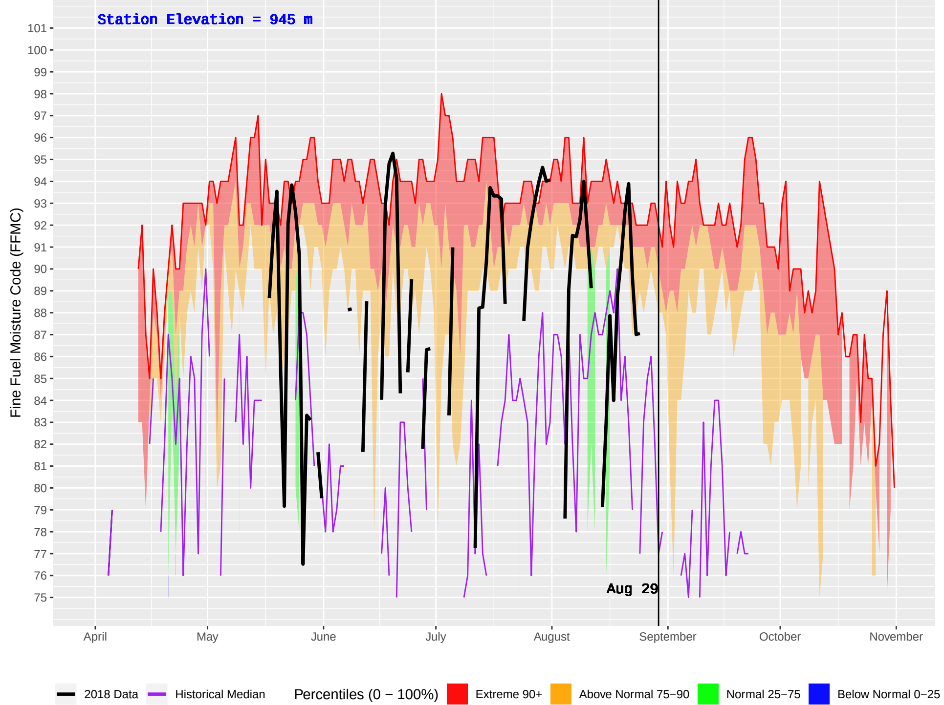
BOWRON HAGGEN (193) : Historical (1986–2016) and Current (2018) Daily Fine Fuel Moisture Code (FFMC)
